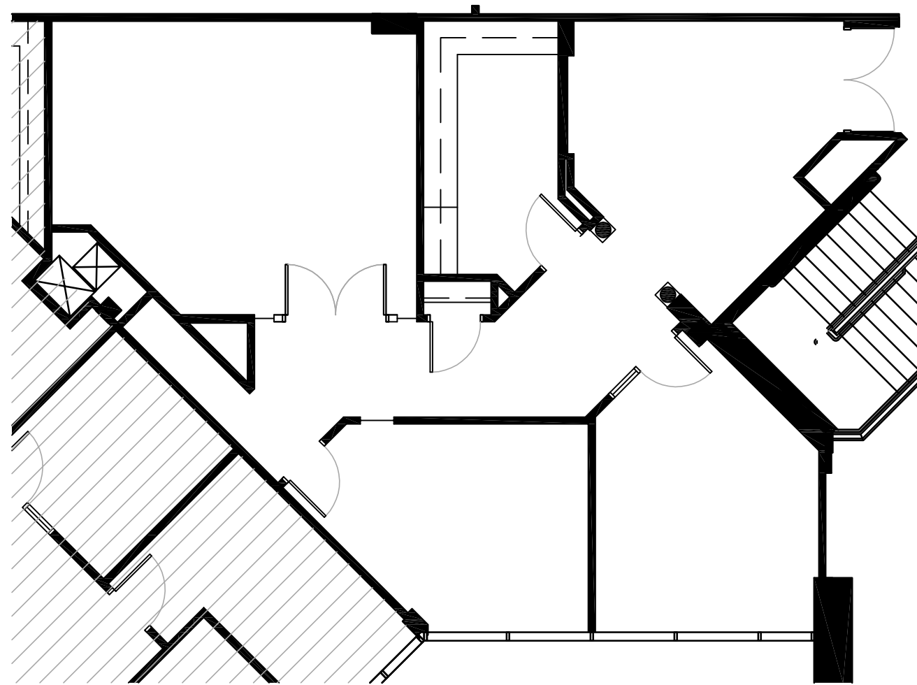
Floor Plan - Second Floor
